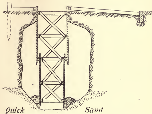
FIG. 28.—SHEATHING A BADLY CAVED TRENCH.
